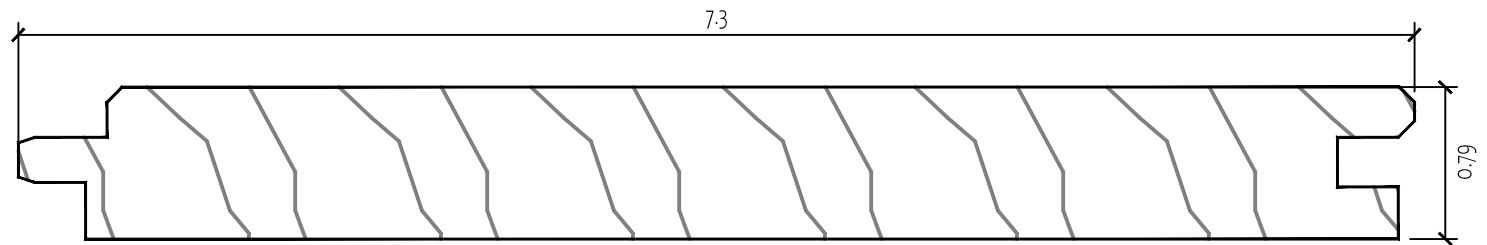
1x8 CLADDING GROOVED C15 (JEM)
