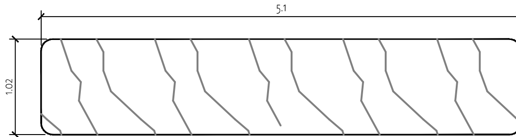
5/4 X 6 STANDARD DECKING - NO GROOVE (JEM)
