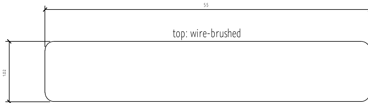
5/4 X 6 Kodiak Spruce No Groove Decking
