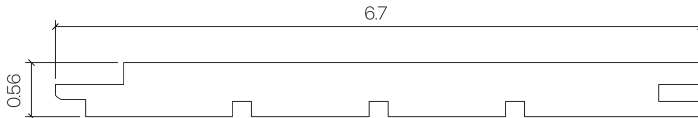
1x7 WALL PANEL - STS10
